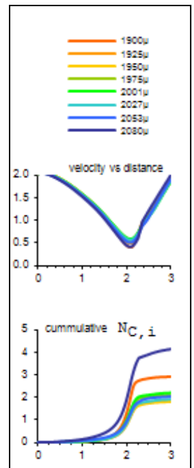
Figure 9: Velocity and Particle Count for various Particle Sizes
